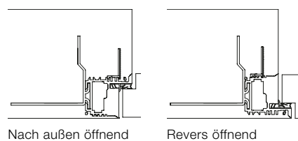
Profile Zeroline-Zarge
